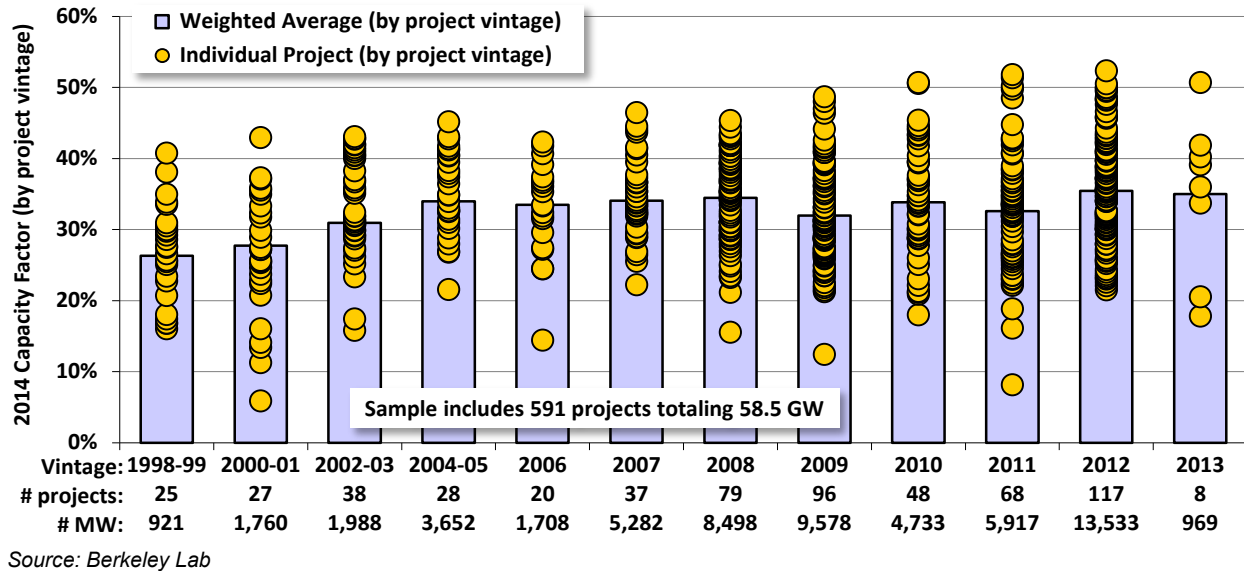
Figure 32. Calendar year 2014 capacity factors by project vintage
