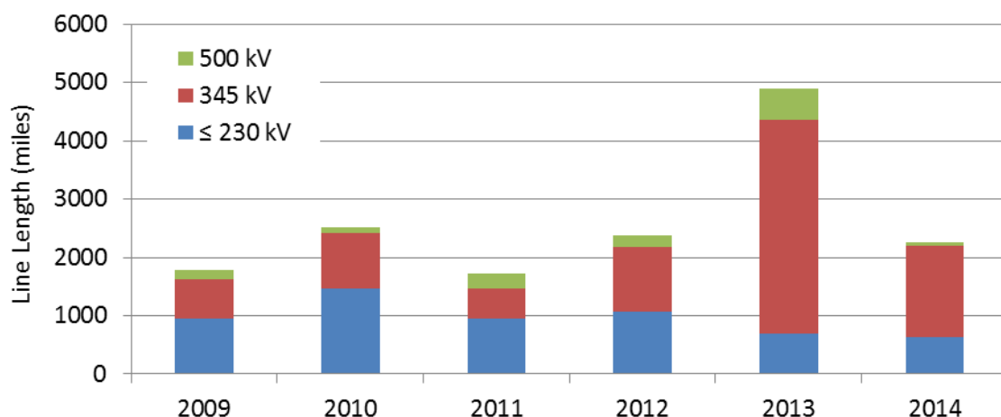
Figure 51. Miles of transmission projects completed, by year and voltage
